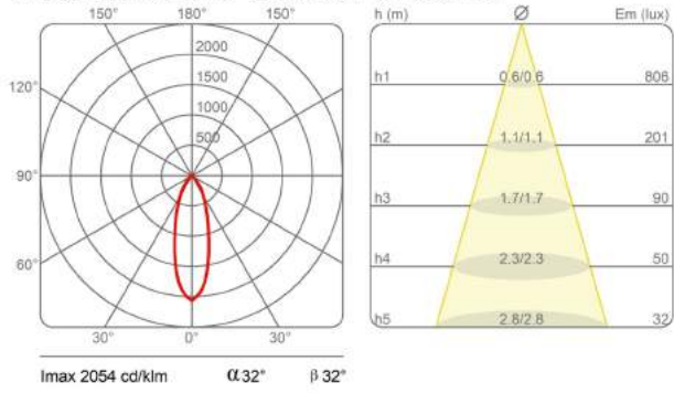
21013/38/NE-DK SISTEMA U - 38° DARKLIGHT13W 3000K LED
